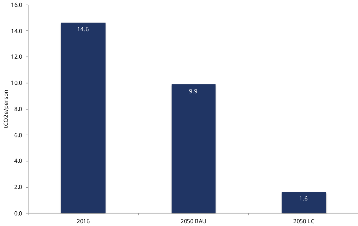
Figure 52. Projected emissions per capita (tCO2e/person), Hamilton.
