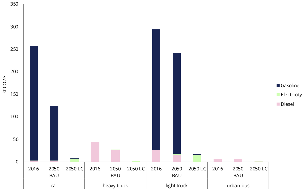
Figure 37. Projected transportation GHG emissions (ktCO 2 e) by source and vehicle type, Burlington.
