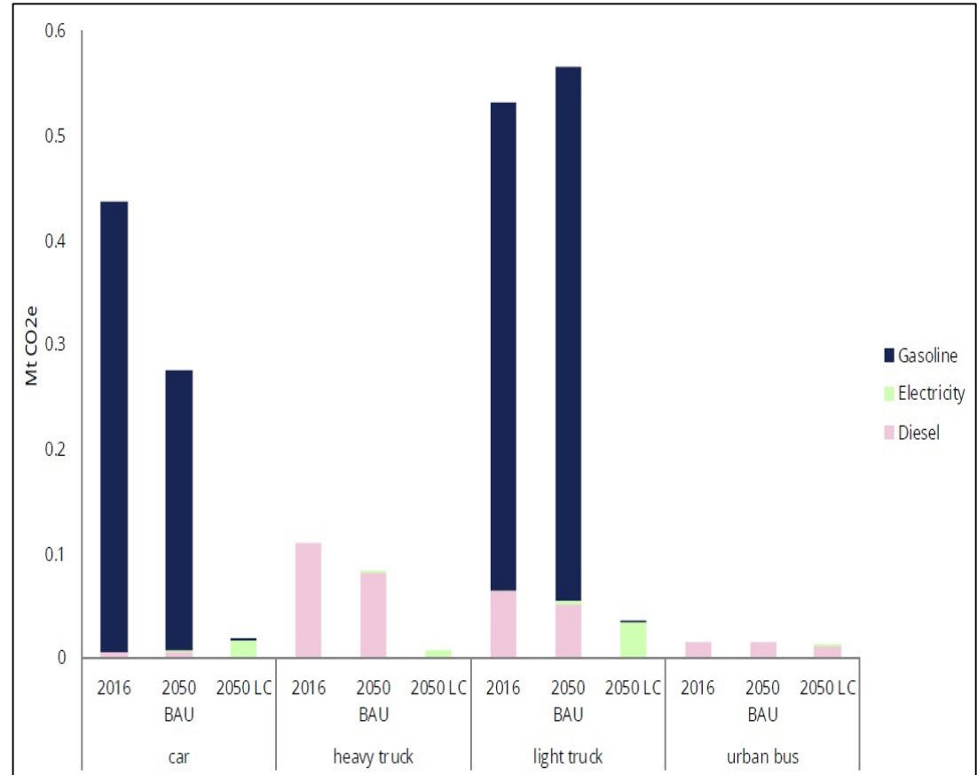
Transportation Emissions by Source & Vehicle Type
