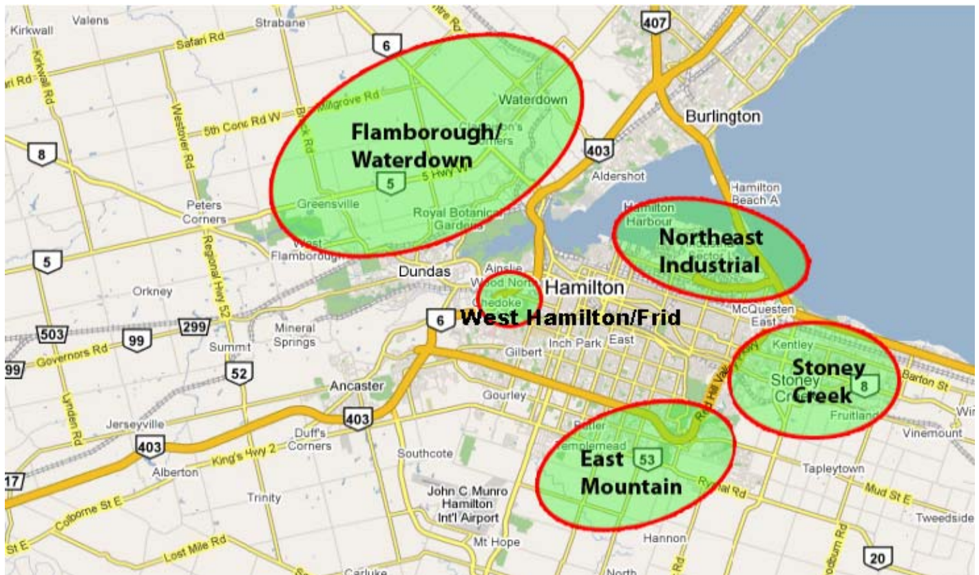
Figure 12: Emission Sources by Region in the Hamilton Area
