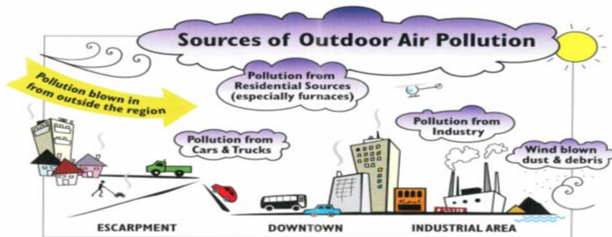
Figure 2: The Air Pollution Picture
