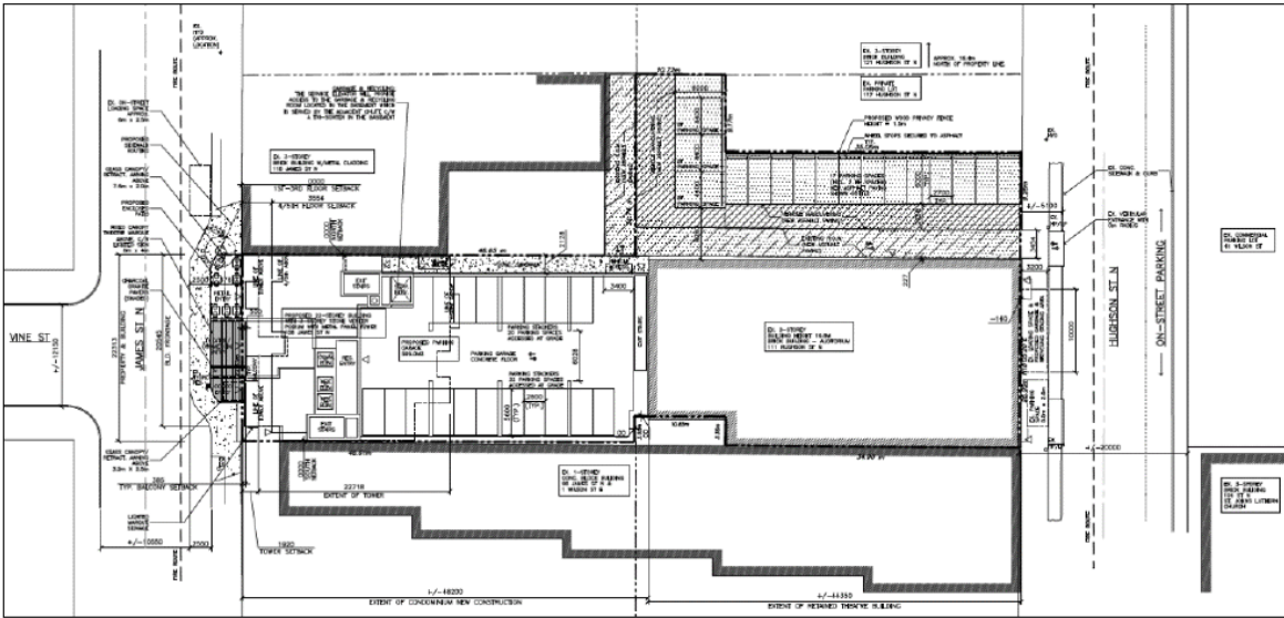
Figure 4: Proposed Site Plan (Source: MSA 2014)
