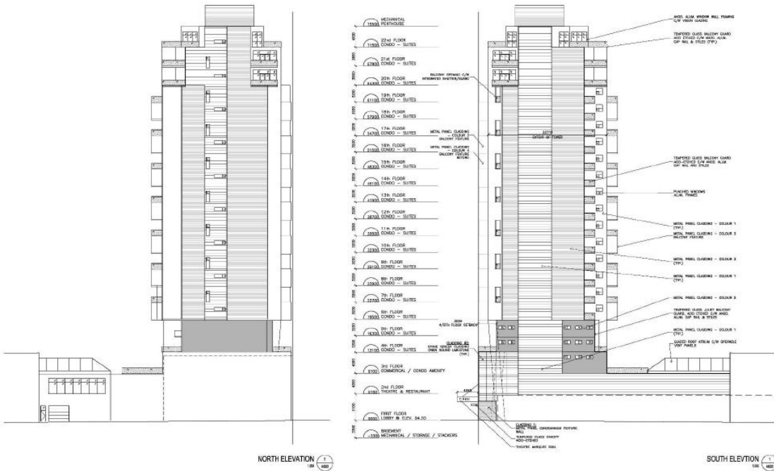
Figure 14: North and South Elevations
