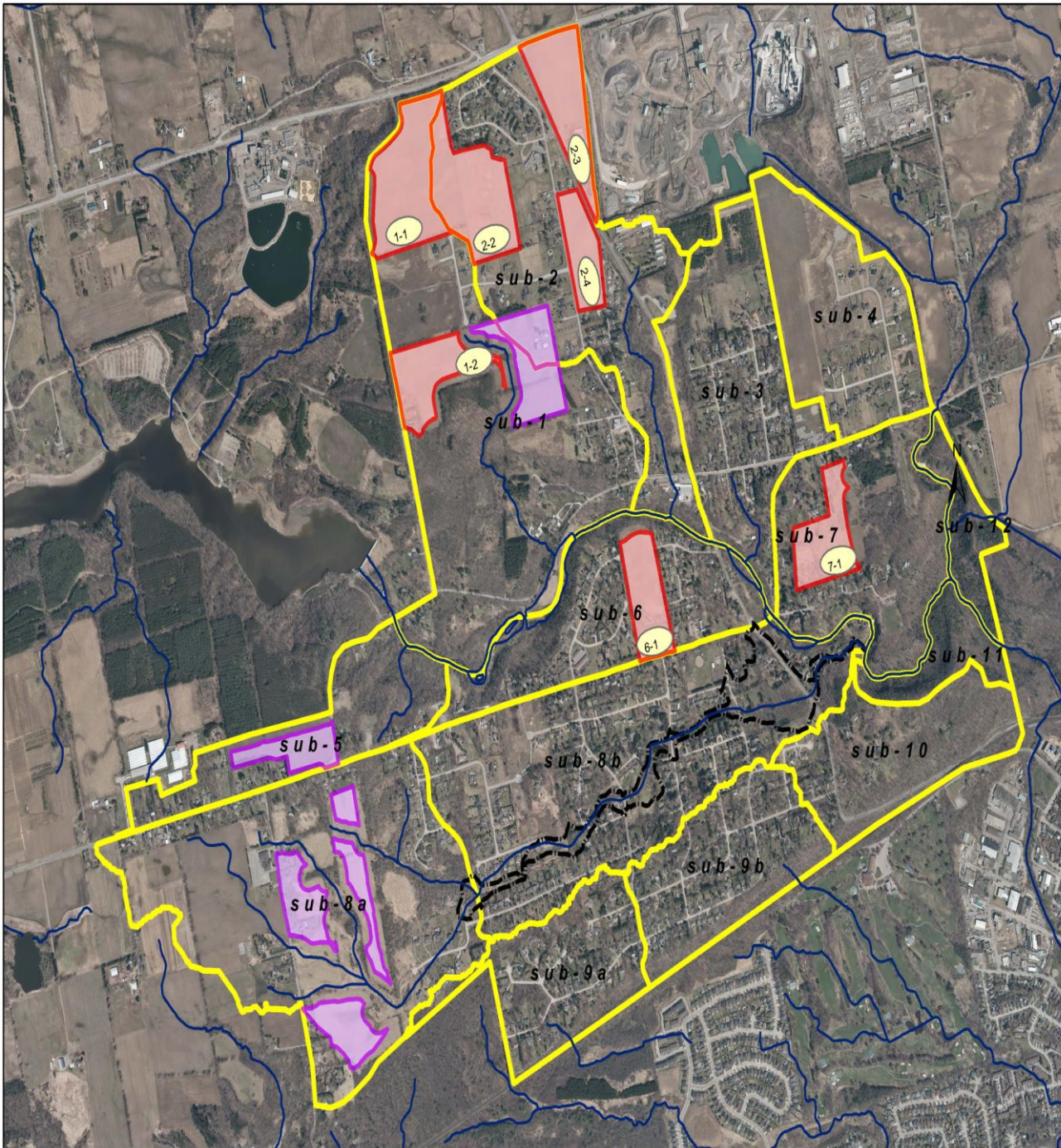
FIGURE 9.2.1 Stormwater Management Facilities for Water Quality /Erosion and Flood Control
