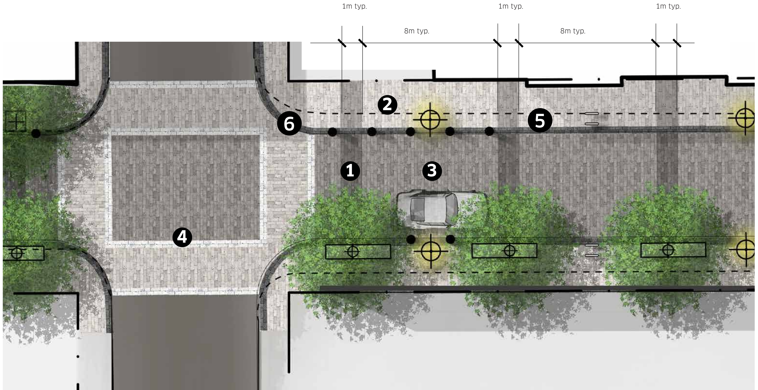
FIGURE 3.4.1.1: PAVING DEMONSTRATION PLAN AT HUGHSON STREET.
