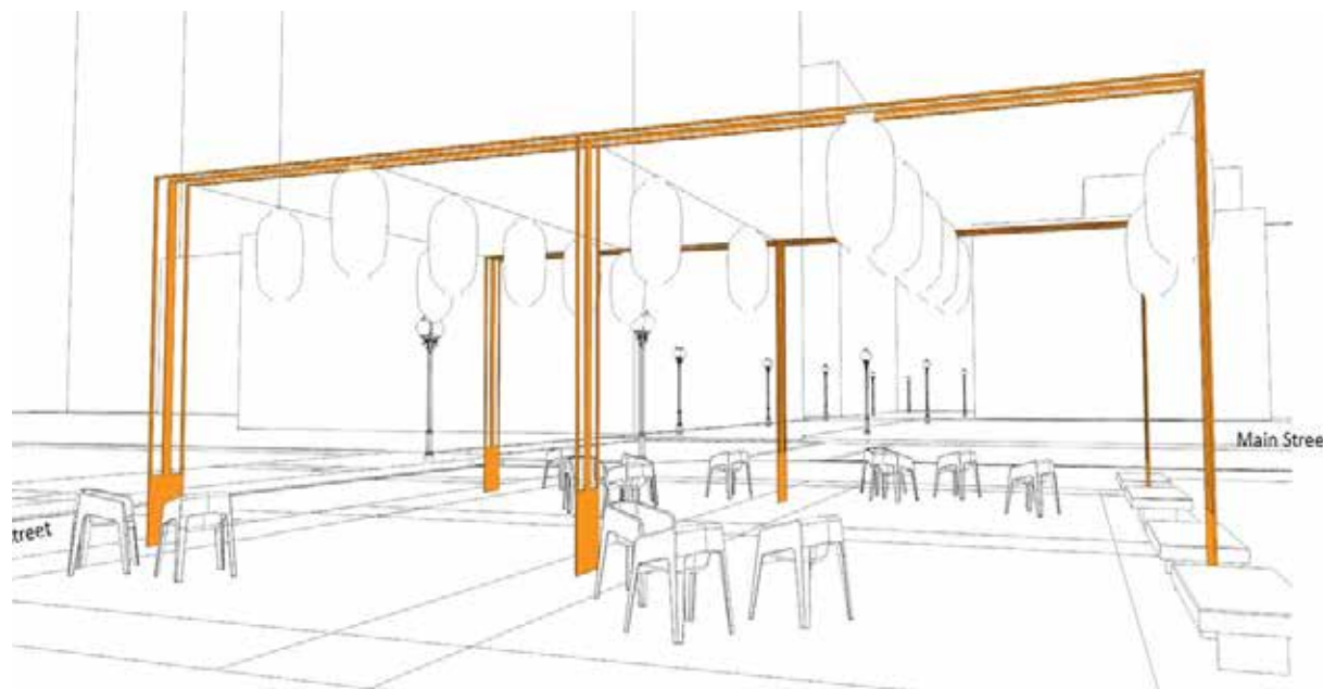
FIGURE 2.4.3.6: PRINCE'S SQUARE PUBLIC PLAZA: CANOPY STRUCTURE CONCEPT
