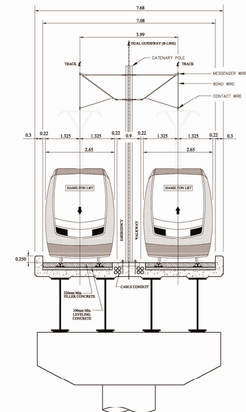
Figure 2.3: Tangent Track Typical Dual Guideway Cross-Section
