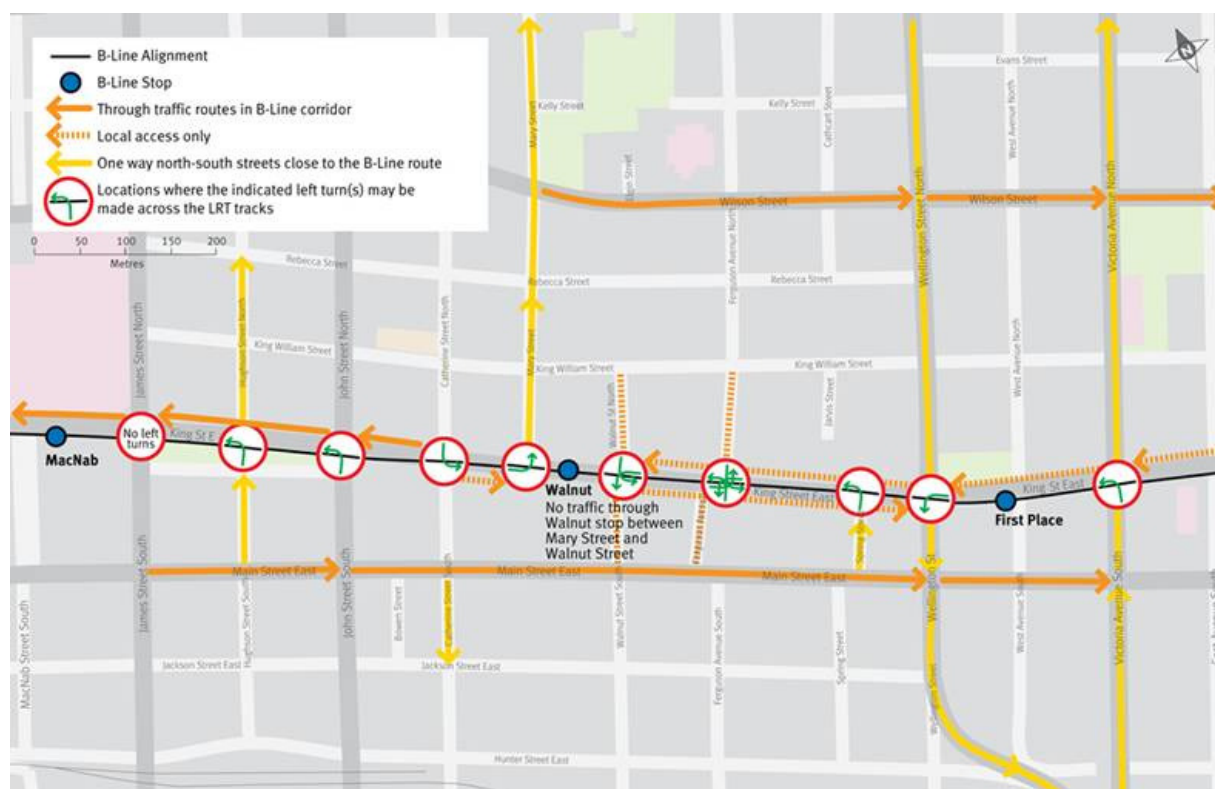
Figure 4.3b: Traffic Circulation
