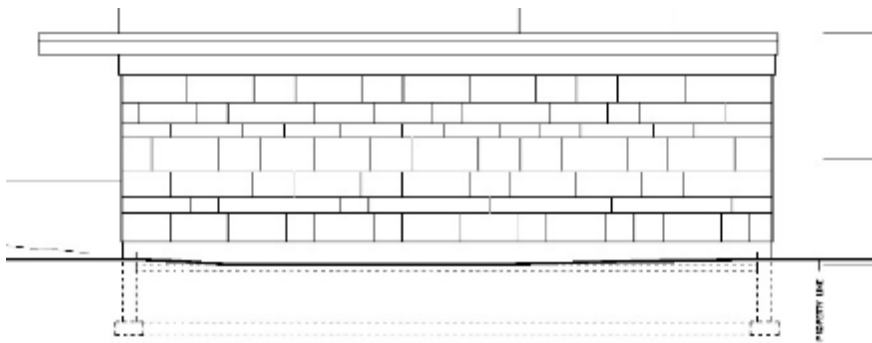
North Elevation (facing laneway)
