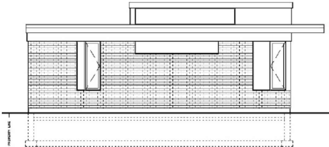
South Elevation (facing existing single detached dwelling)
