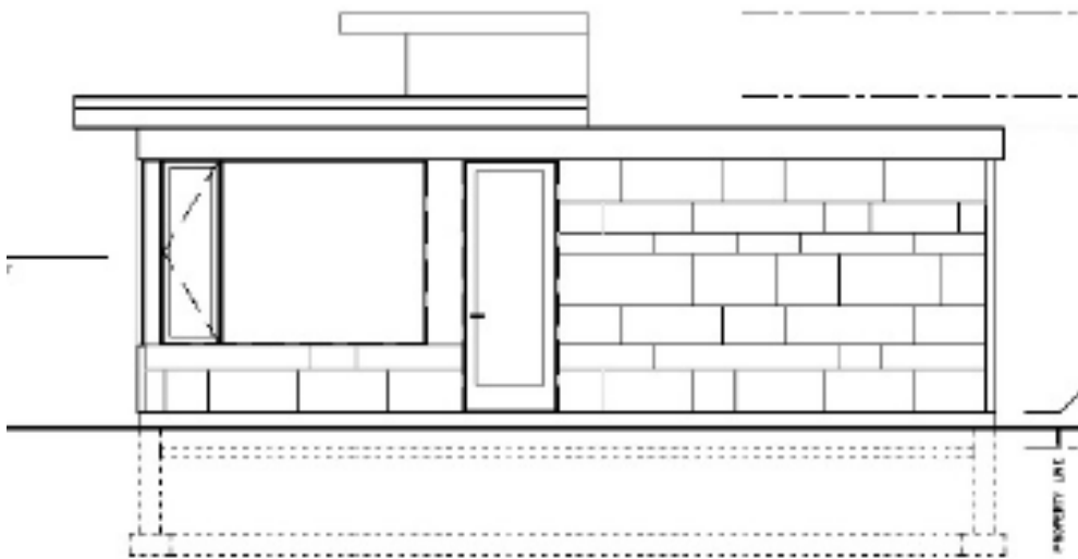
East Elevation (facing proposed patio area)
