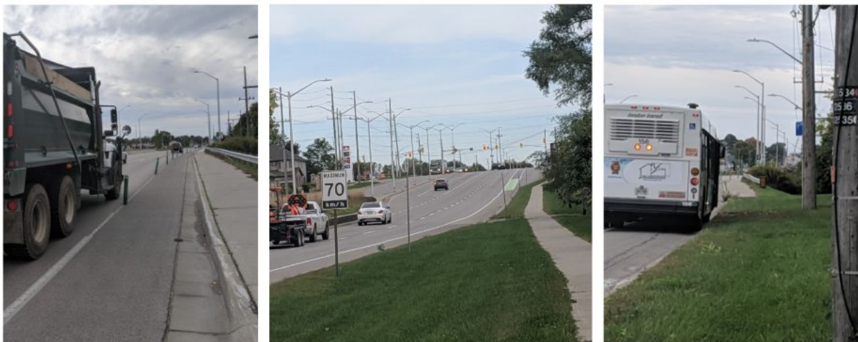
Figure 5-2: Painted and bollard bike lanes on Highbury Ave between Killarney Rd and Edgevalley Rd. installed in 2018. Posted speed limit 70km/h, 4 traffic lanes. When cyclists mix with traffic at 60km/h or more, the risk of a collision causing catastrophic injury or death in London is 27% - or 1 in 4 38 . Left plate shows broken bollards from collisions with vehicles. The bollards are completely removed in the winter when the bike lane is used for snow storage. Middle plate shows cyclists share the road with large trucks and buses at high speeds. Right plate shows planned bus stop in
