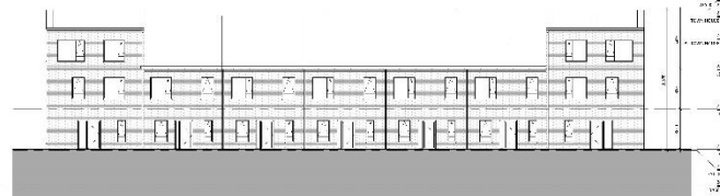
⑦ GROUP 4 WEST ELEVATION 1/8" = 1' - 0"
