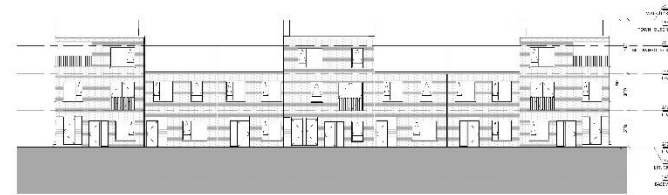
① GROUP 3 NORTH ELEVATION 1/8" = 1' - 0"
