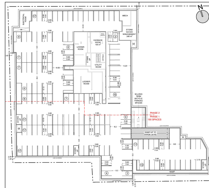
UNDERGROUND PARKING - SCALE 1:400
