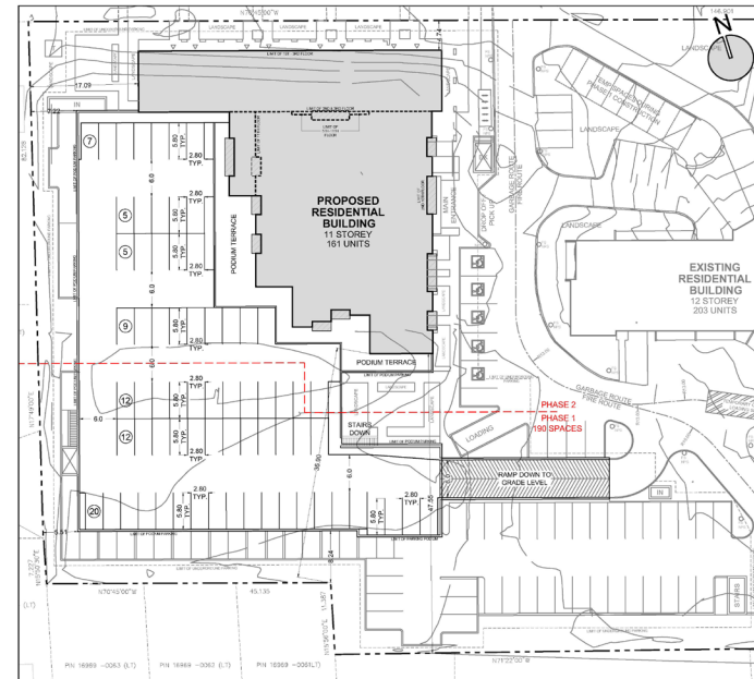
PODIUM PARKING - SCALE 1:400
