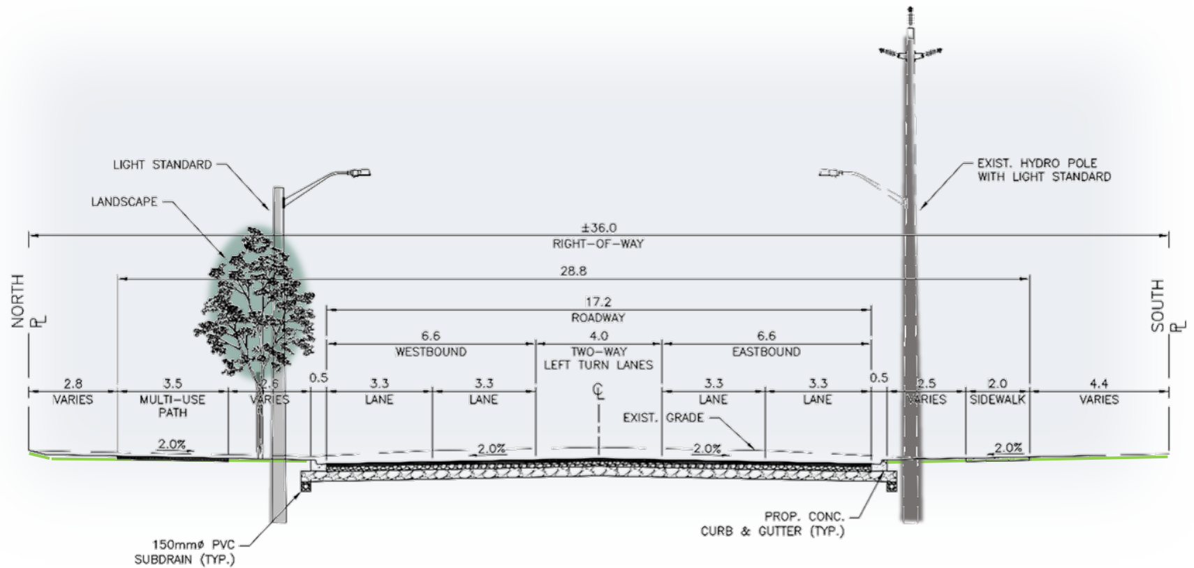
TYPICAL CROSS-SECTION
