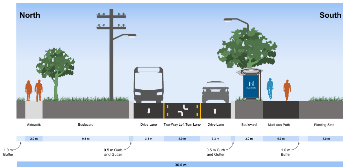
Figure 2. Recommended Design Concept for Barton Street from Lewis Road to Fifty Road
