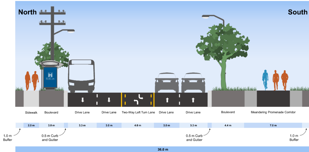
Figure 1. Recommended Design Concept for Barton Street from Fruitland Road to Fifty Road
