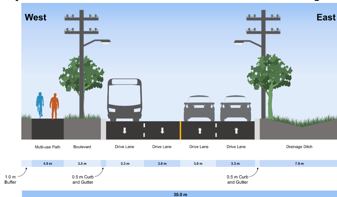
Figure 4. Recommended Design Concept for Fifty Road from Barton Street to South Service Road
