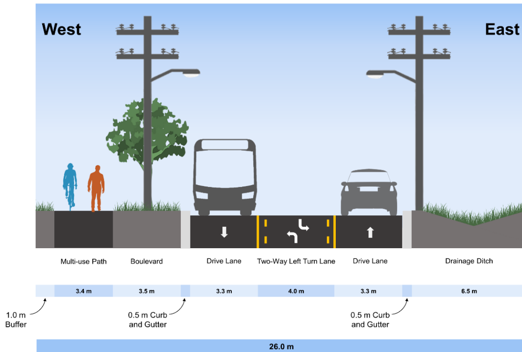
Figure 3. Recommended Design Concept for Fifty Road from Highway 8 to Barton Street
