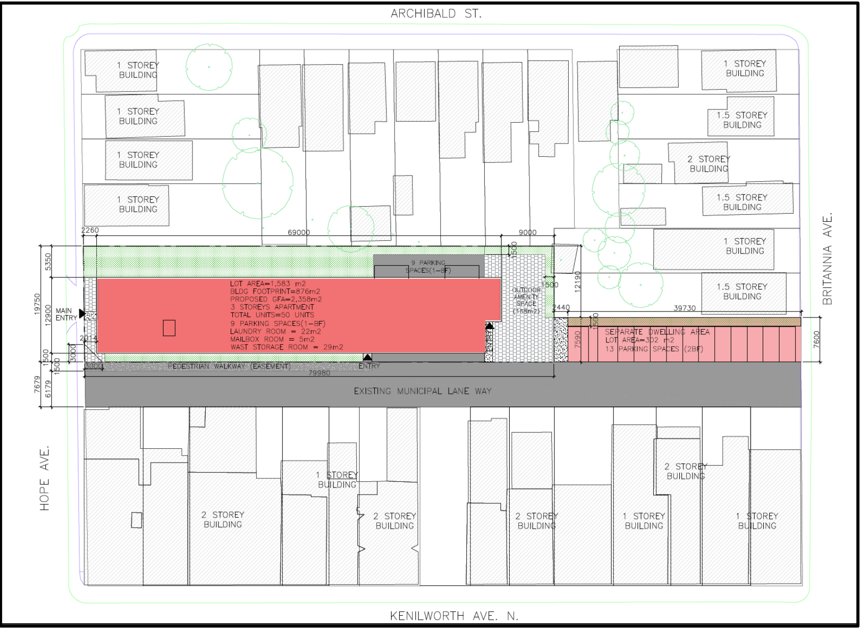
Figure 1: Apartment Concept
